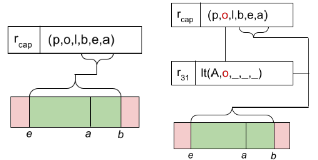
(b) A borrowed capability only carries authority over memory if register 31 contains a matching lifetime token.
